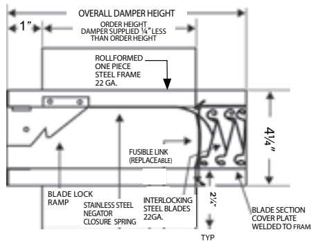
(H) HORIZONTAL MOUNT
