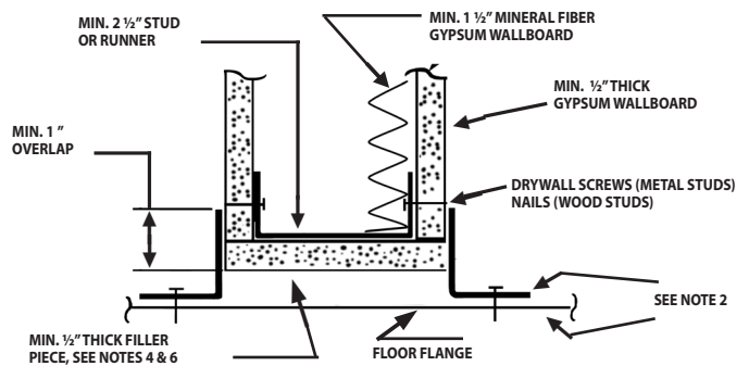
1-HOUR RATED PARTITION WALL SECTION "B-B"
