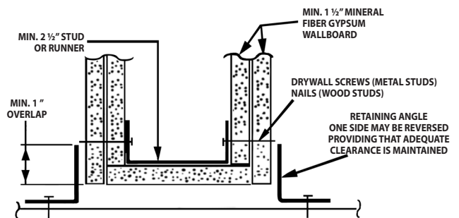
1-HOUR RATED PARTITION WALL SECTION "B-B"
