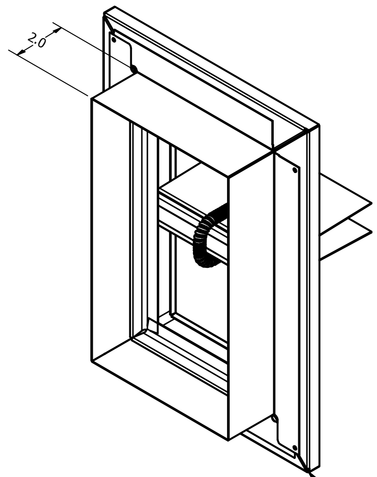
ISOMETRIC VIEW 58EAD
