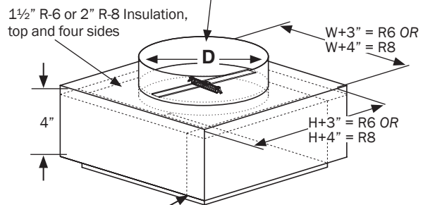
Drywall flange surrounds register opening (W, (≤H) x H) D = Collar, Inlet, CRD Diameter
